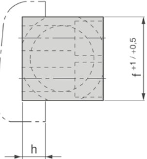
Passung / Seat
