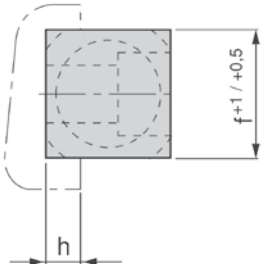
Passung / Seat
