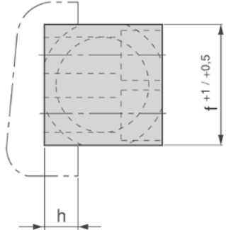
Passung / Seat
